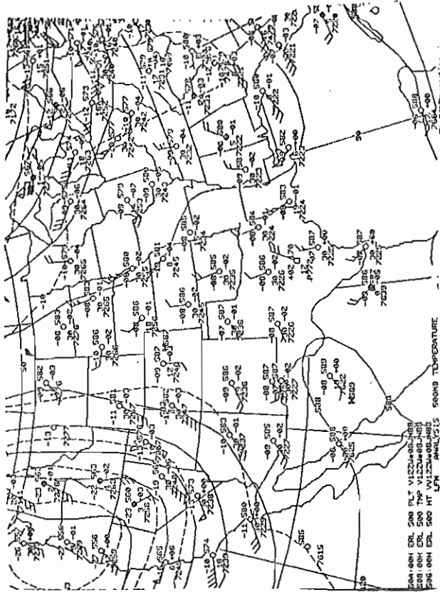
Figure 9 - 500 MB Chart 12 GMT, June 8, 1988
