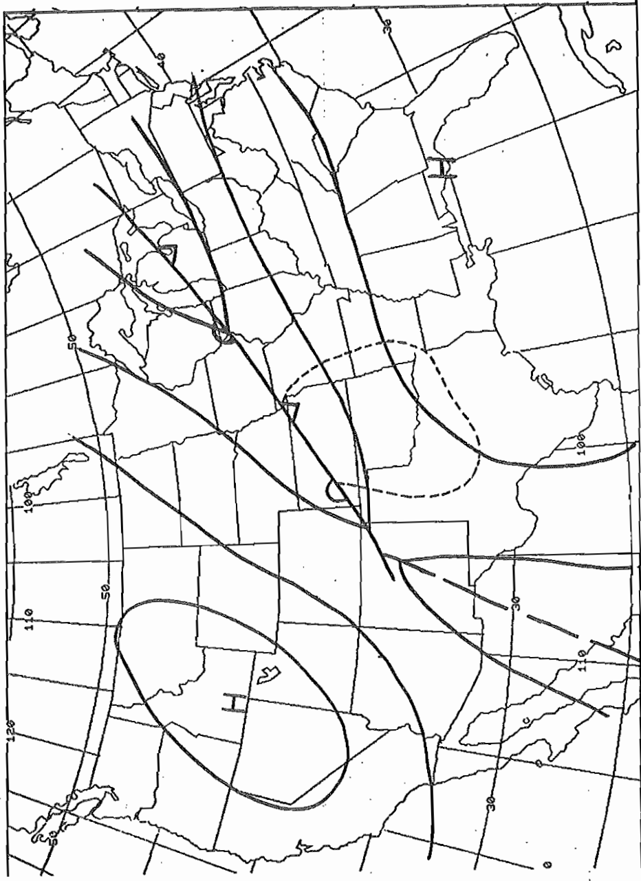
Figure 6 - Surface Chart #1 Solid Lines - Isobars Dashed Line - Outlines Area of Hottest Temperatures
